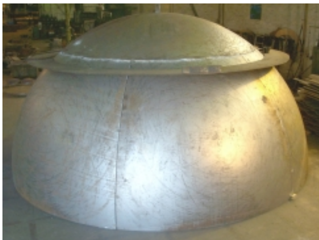
Hemisphere with diameter 6,5 meter.
